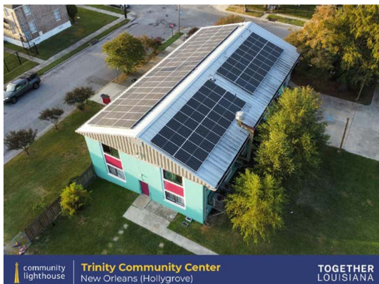
(Left) The Community Lighthouse Project is a planned network of 85 congregations and community institutions across the city that will serve as resilience hubs, providing commercial-grade solar power and backup battery capacity during a power outage or natural disaster. Courtesy of Together New Orleans.
